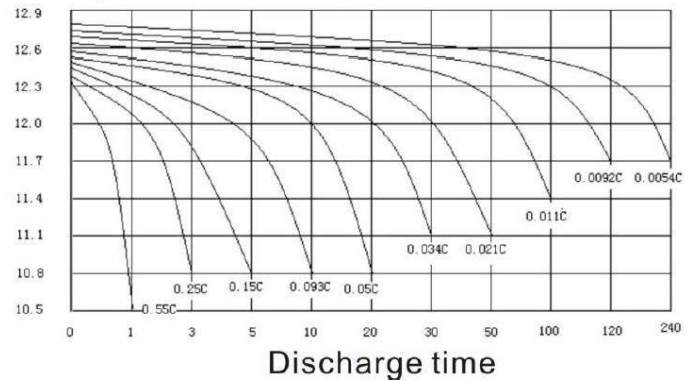
Discharge performance
